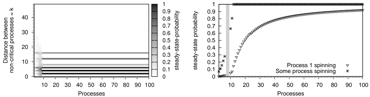
Figure 4: The left diagram shows the steady-state probabilities that at a given moment there are exactly k processes in their non-critical section. Darker grey indicates higher probability, as indicated in the legend. The right diagram shows the steady-state probabilities that at a given moment (1) process P_1 is “spinning”, i.e., waiting for the lock and (2) that at least one process is “spinning”. 2 to 100 processes.
